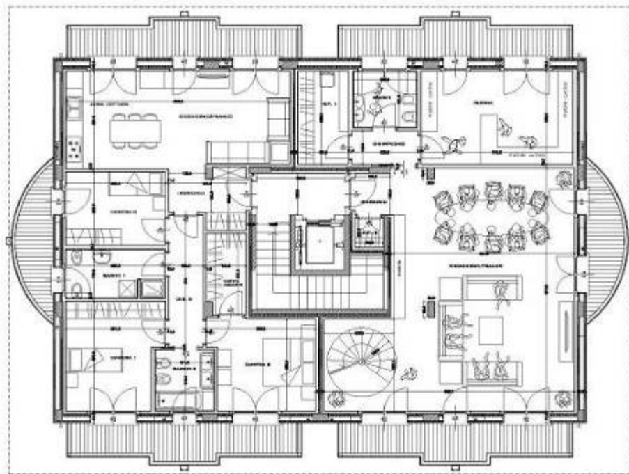
PIANTA PIANO 5
